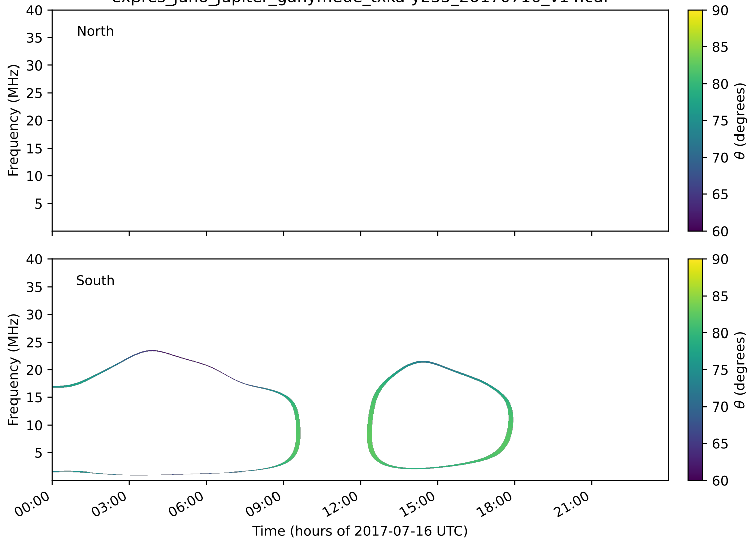
expres_juno_jupiter_ganymede_txka-y235_20170716_v14.cdf
