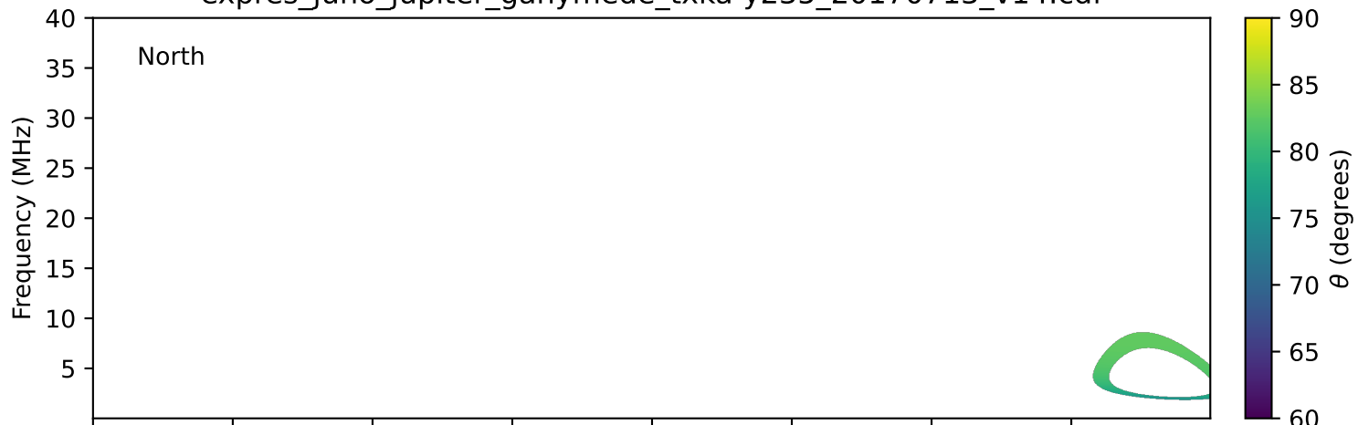
expres_juno_jupiter_ganymede_txka-y235_20170713_v14.cdf
