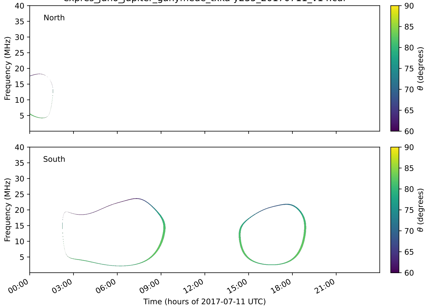
expres_juno_jupiter_ganymede_txka-y235_20170711_v14.cdf
