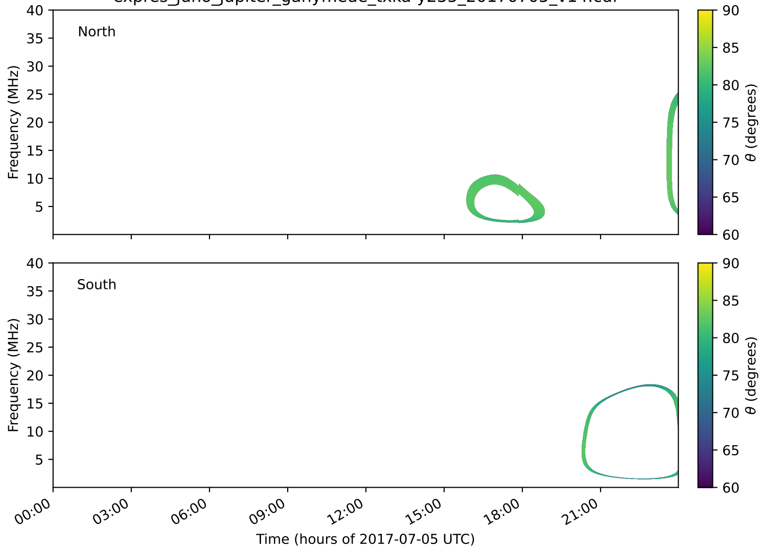
expres_juno_jupiter_ganymede_txka-y235_20170705_v14.cdf
