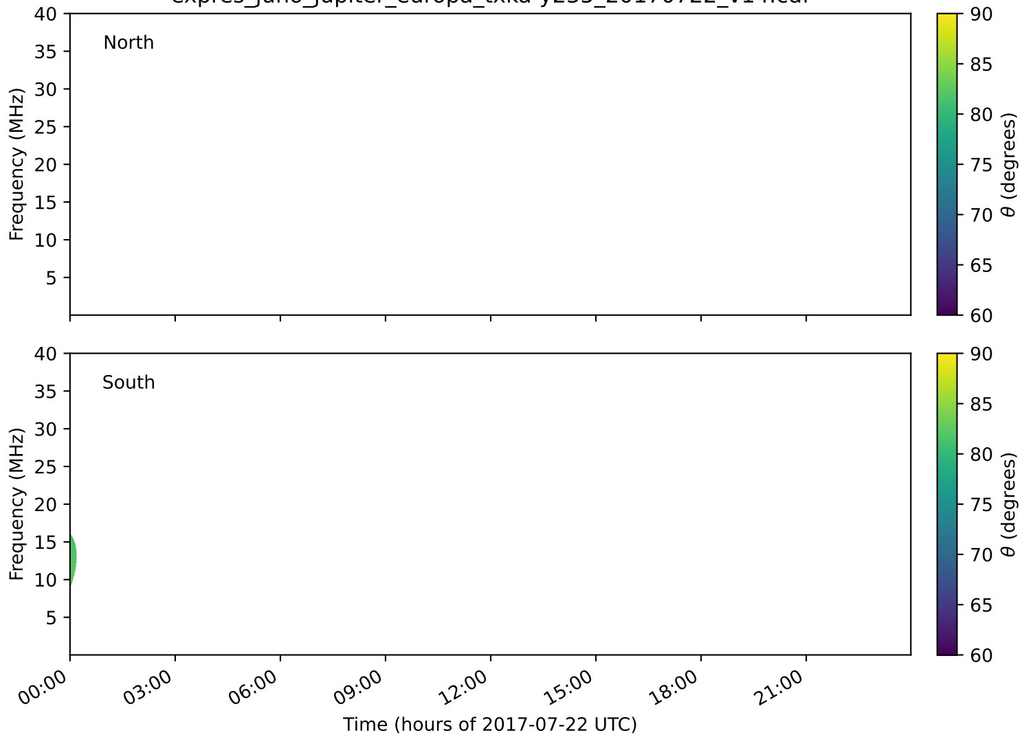
expres_juno_jupiter_europa_txka-y235_20170722_v14.cdf
