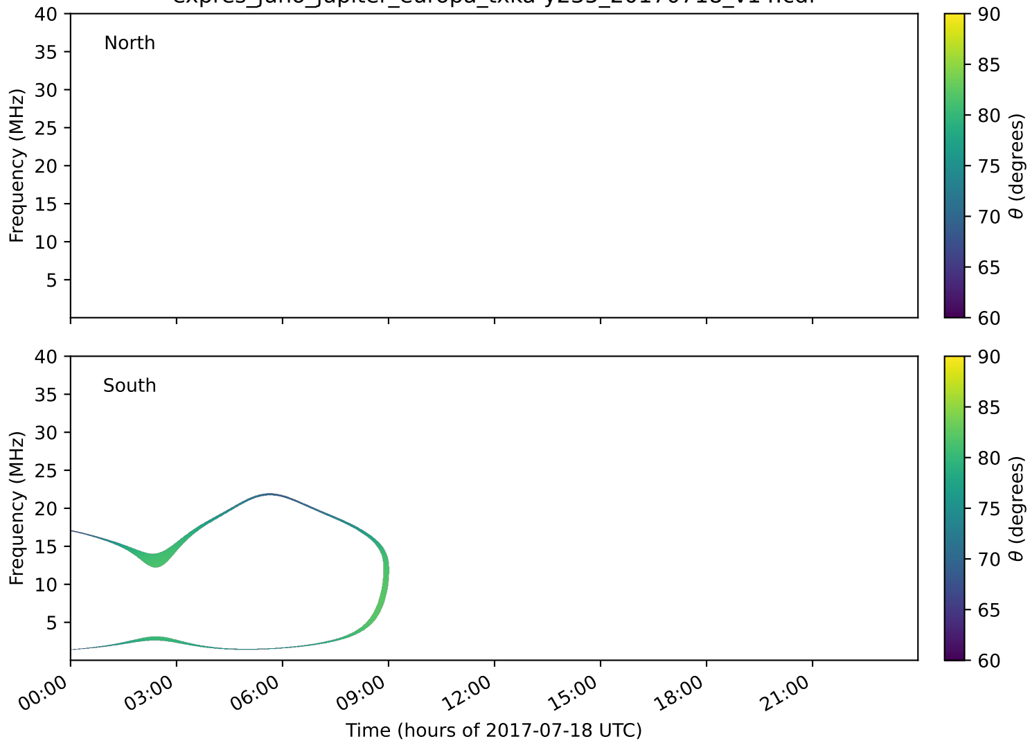
expres_juno_jupiter_europa_txka-y235_20170718_v14.cdf
