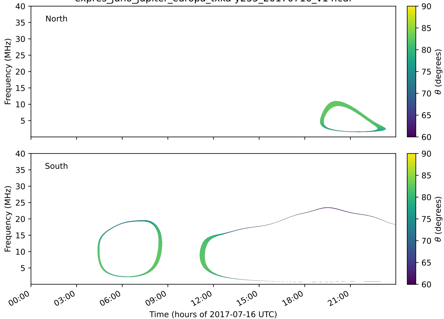
expres_juno_jupiter_europa_txka-y235_20170716_v14.cdf
