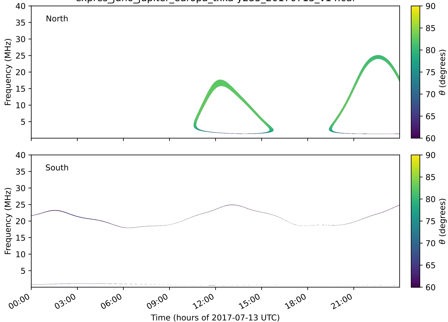
expres_juno_jupiter_europa_txka-y235_20170713_v14.cdf
