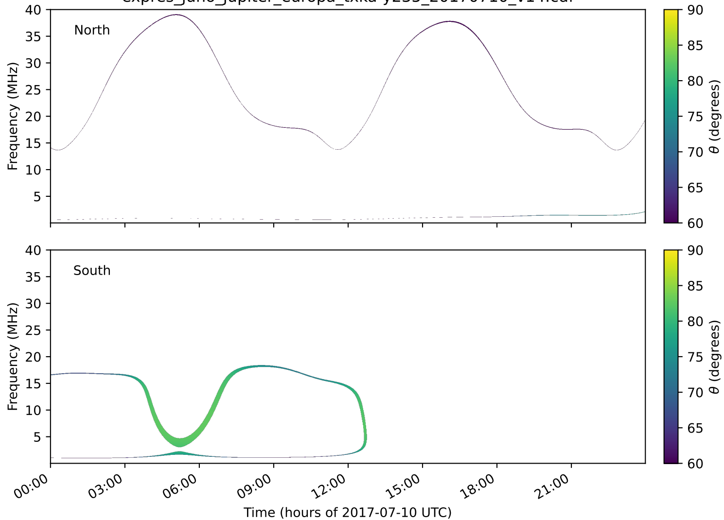
expres_juno_jupiter_europa_txka-y235_20170710_v14.cdf
