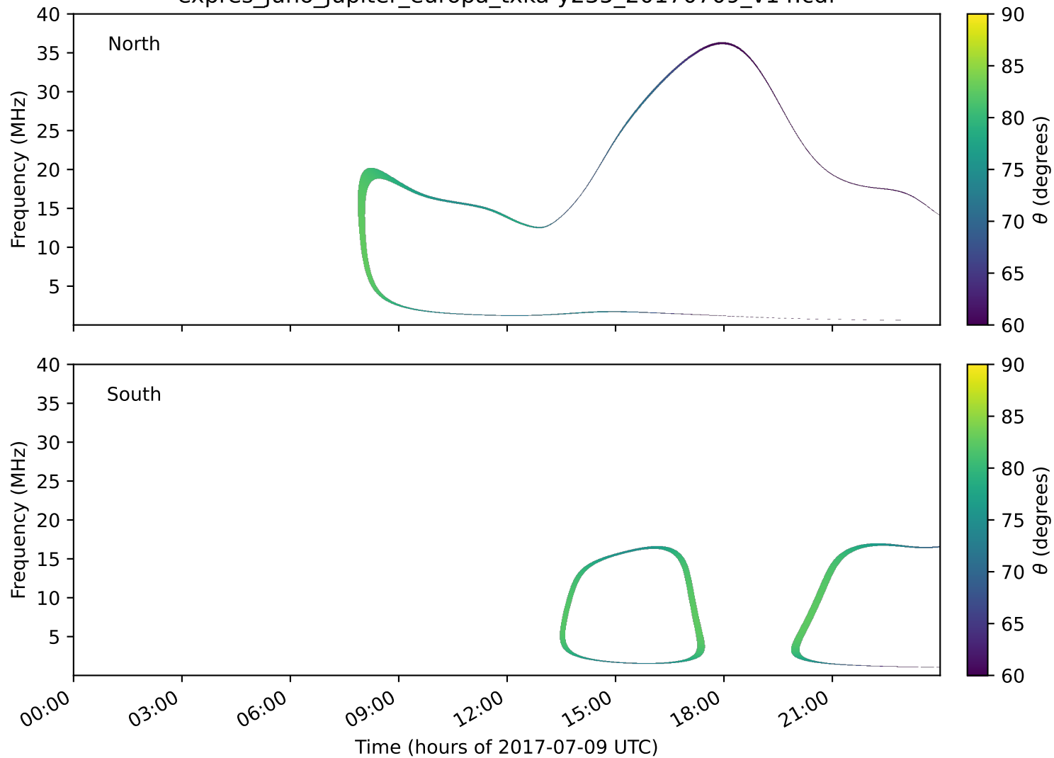
expres_juno_jupiter_europa_txka-y235_20170709_v14.cdf
