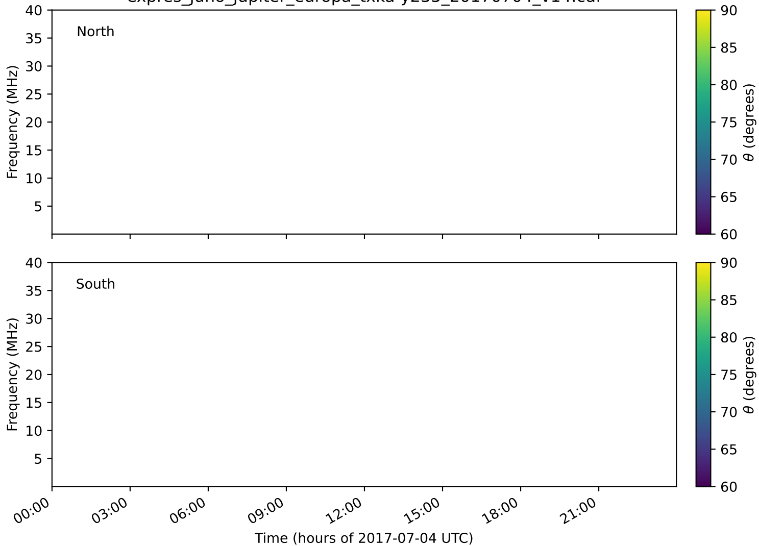
expres_juno_jupiter_europa_txka-y235_20170704_v14.cdf
