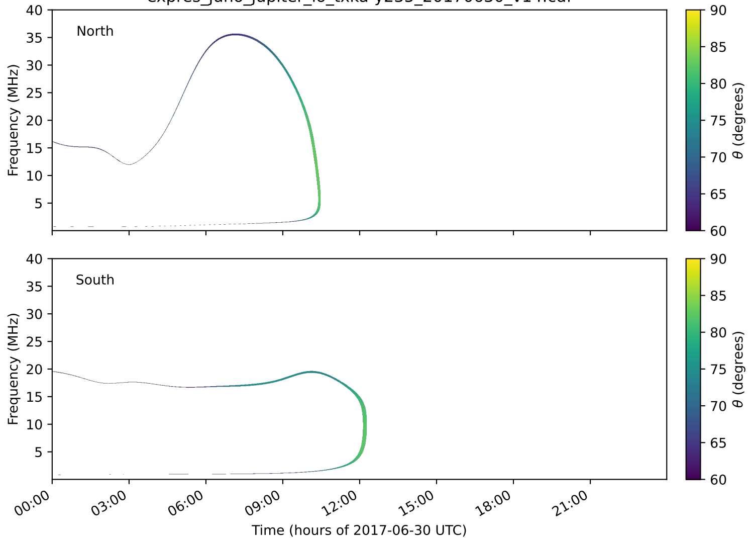
expres_juno_jupiter_io_txka-y235_20170630_v14.cdf
