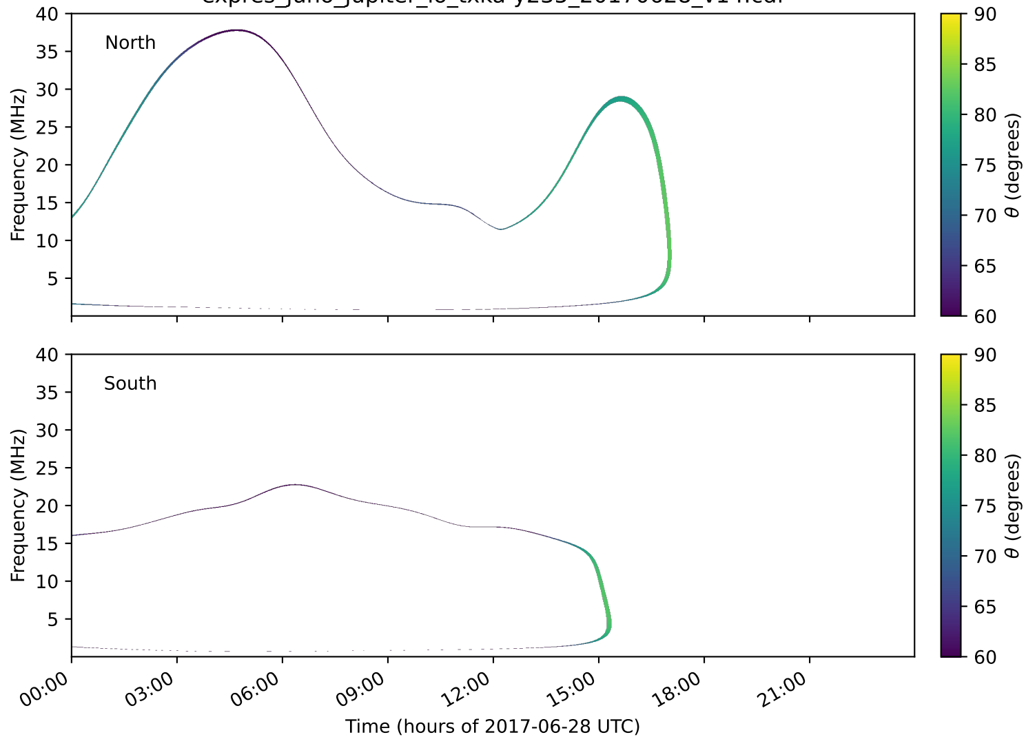
expres_juno_jupiter_io_txka-y235_20170628_v14.cdf
