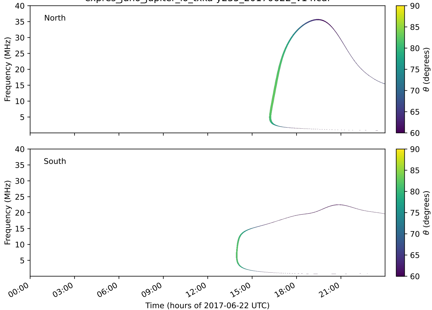
expres_juno_jupiter_io_txka-y235_20170622_v14.cdf
