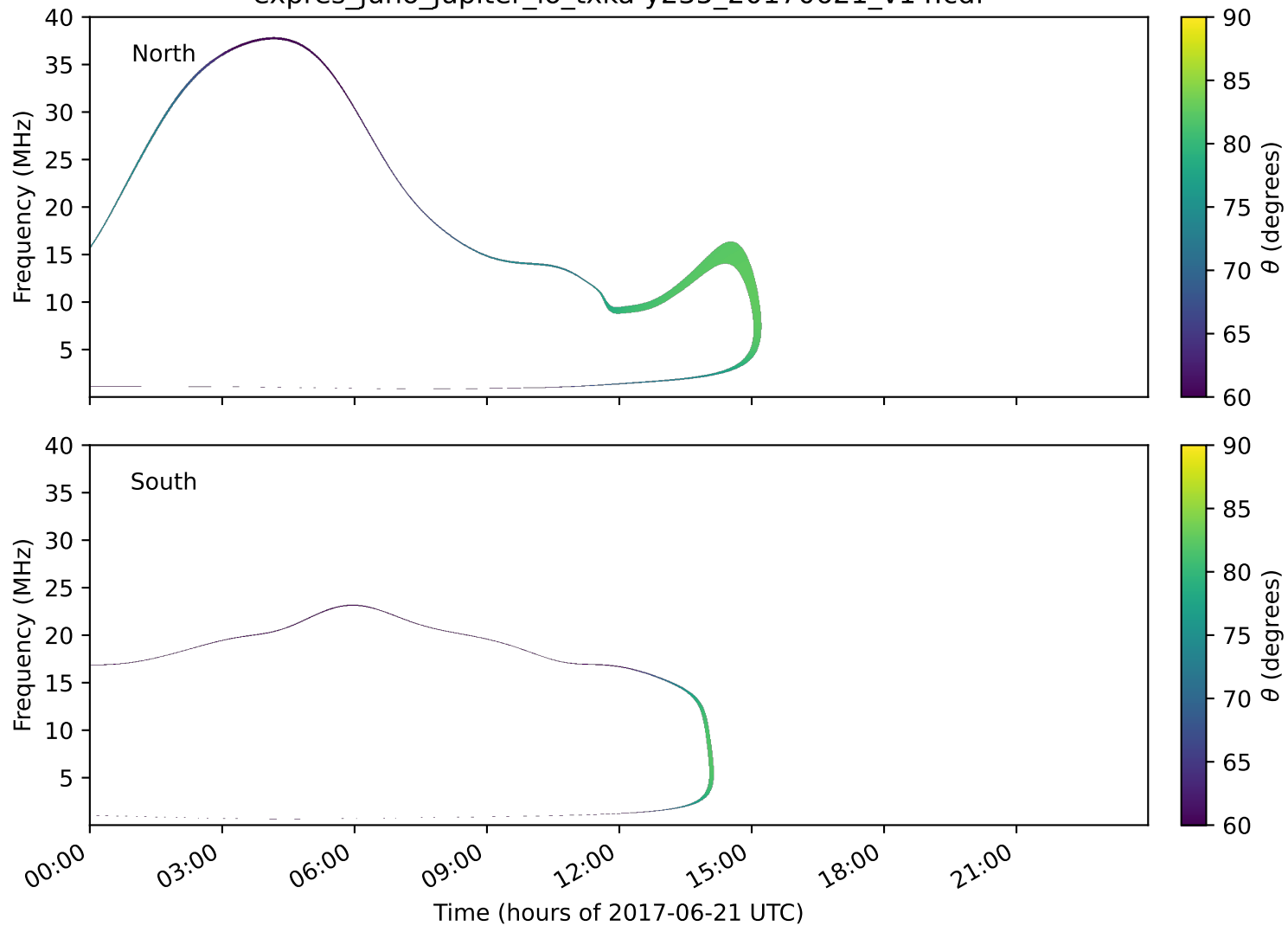
expres_juno_jupiter_io_txka-y235_20170621_v14.cdf
