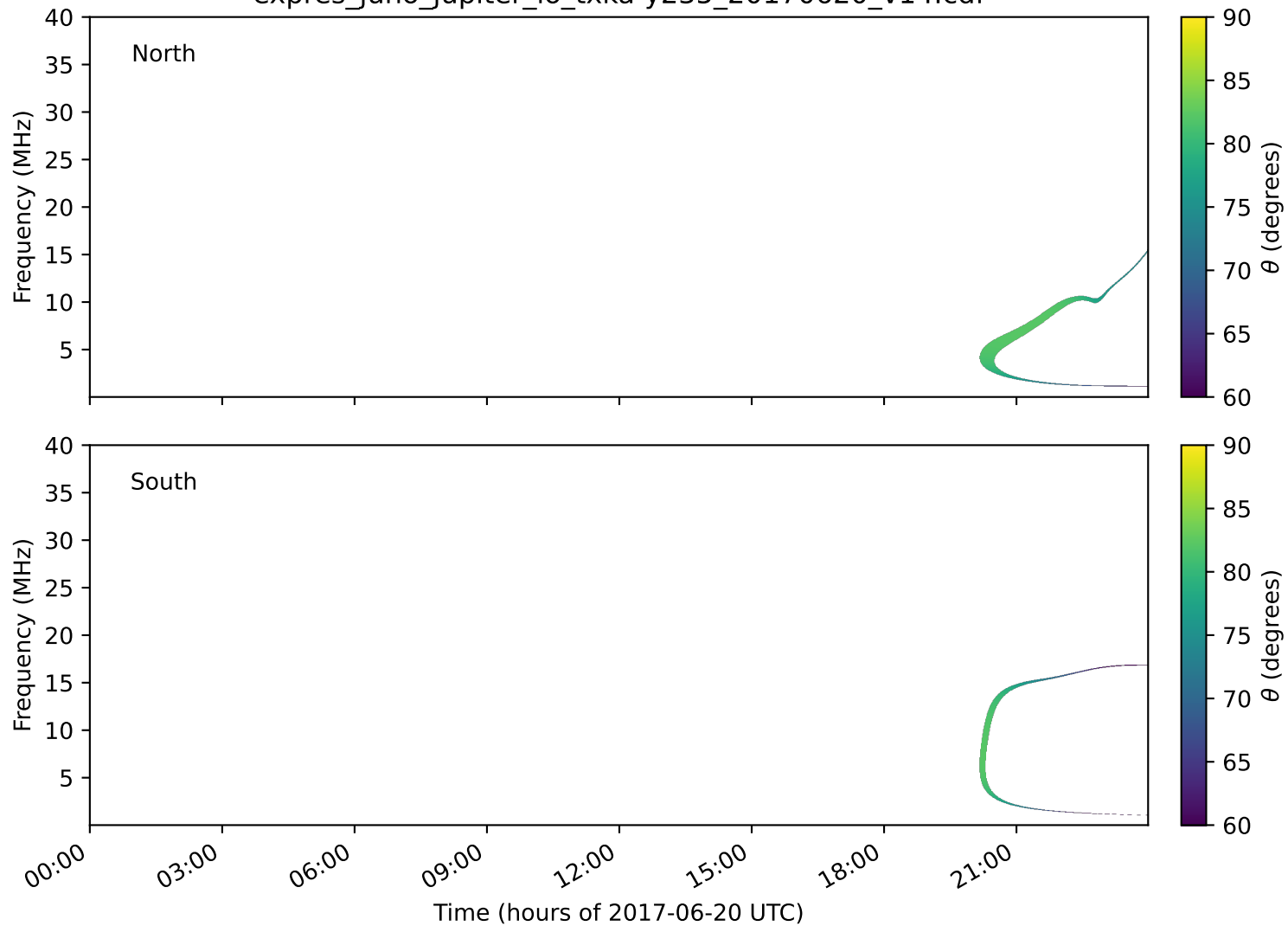
expres_juno_jupiter_io_txka-y235_20170620_v14.cdf
