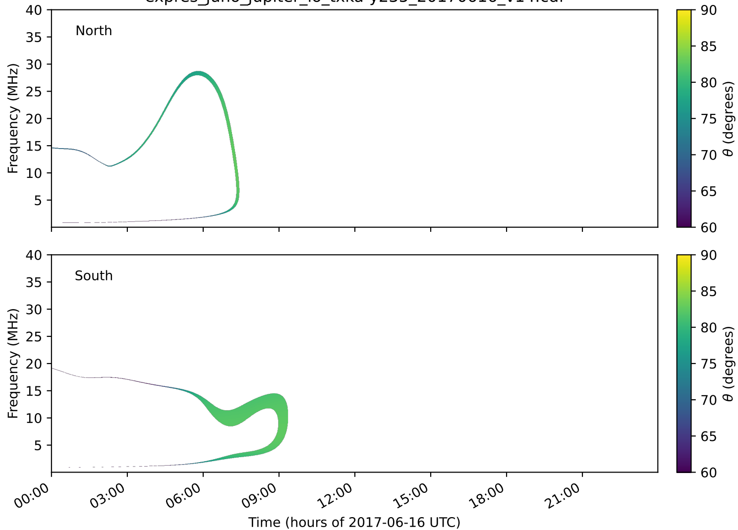
expres_juno_jupiter_io_txka-y235_20170616_v14.cdf
