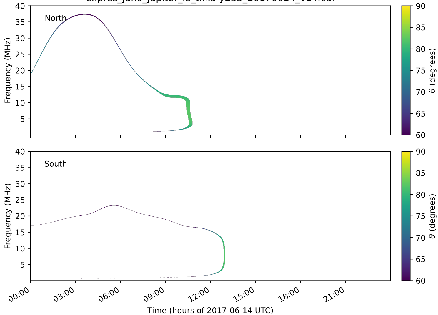
expres_juno_jupiter_io_txka-y235_20170614_v14.cdf
