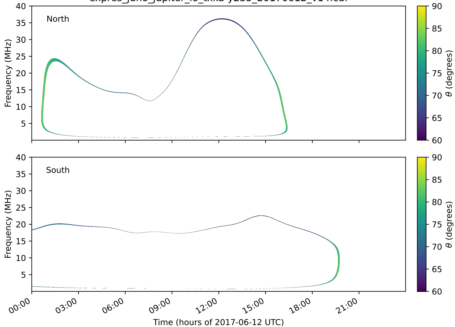
expres_juno_jupiter_io_txka-y235_20170612_v14.cdf
