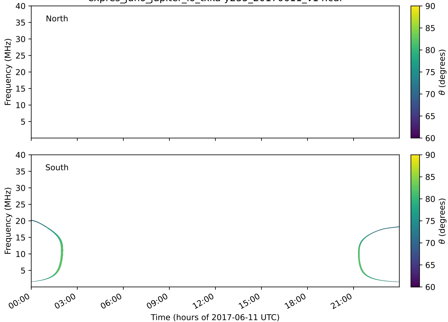
expres_juno_jupiter_io_txka-y235_20170611_v14.cdf
