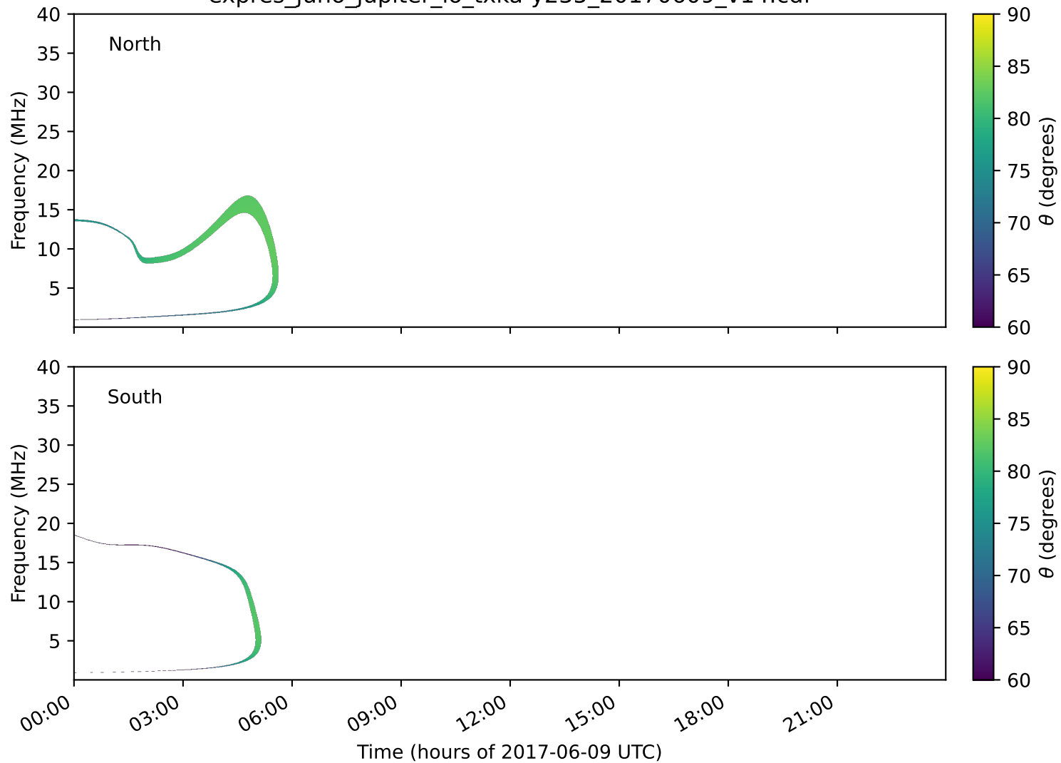
expres_juno_jupiter_io_txka-y235_20170609_v14.cdf
