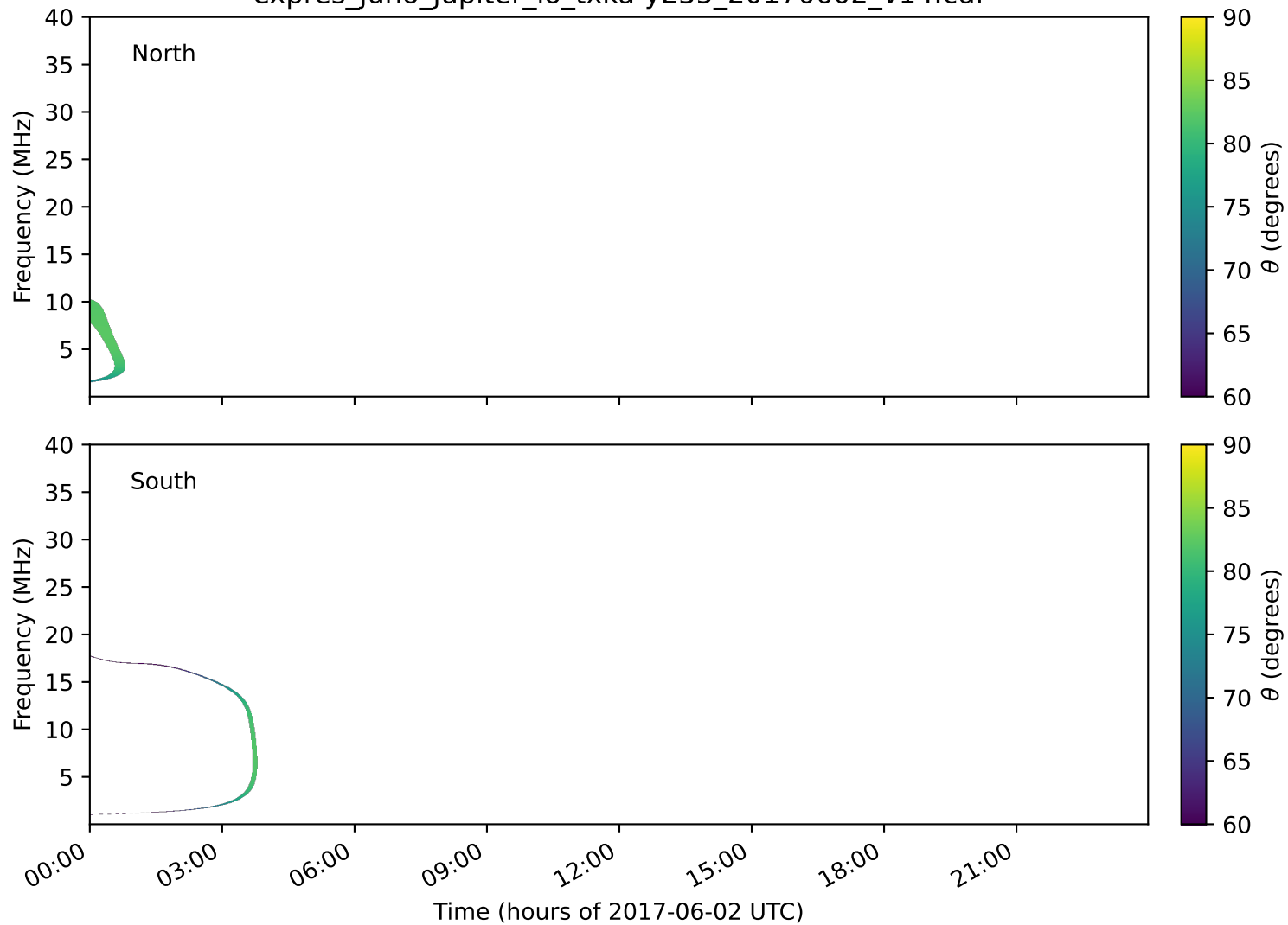
expres_juno_jupiter_io_txka-y235_20170602_v14.cdf
