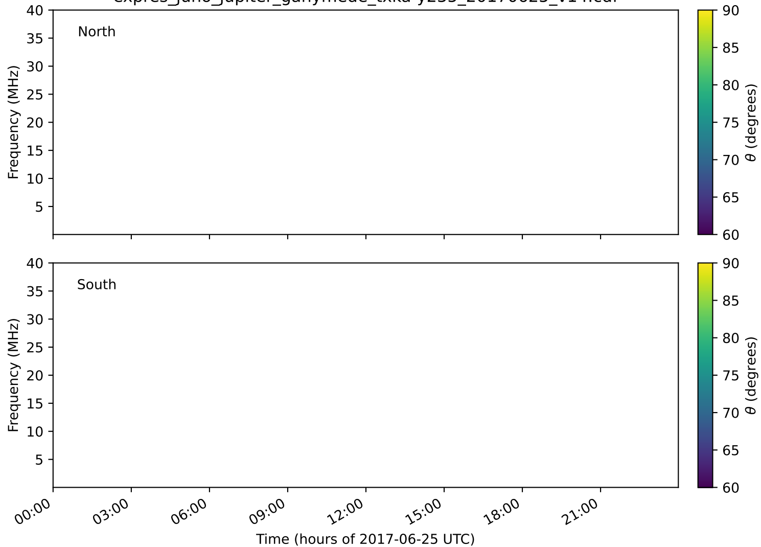
expres_juno_jupiter_ganymede_txka-y235_20170625_v14.cdf
