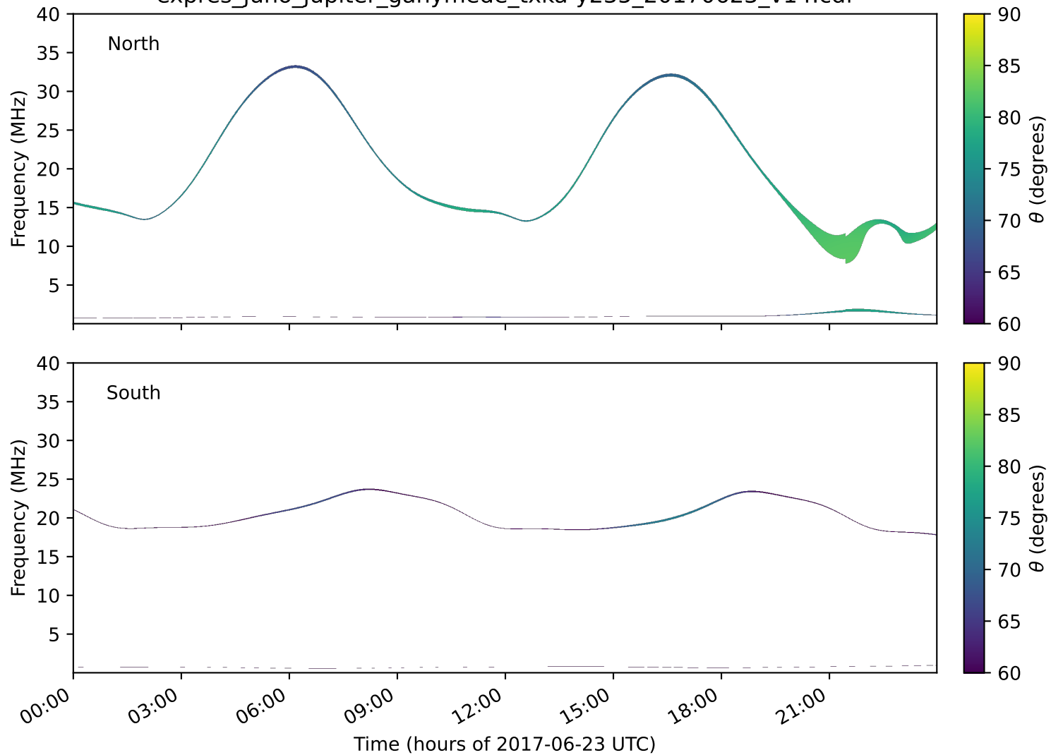
expres_juno_jupiter_ganymede_txka-y235_20170623_v14.cdf
