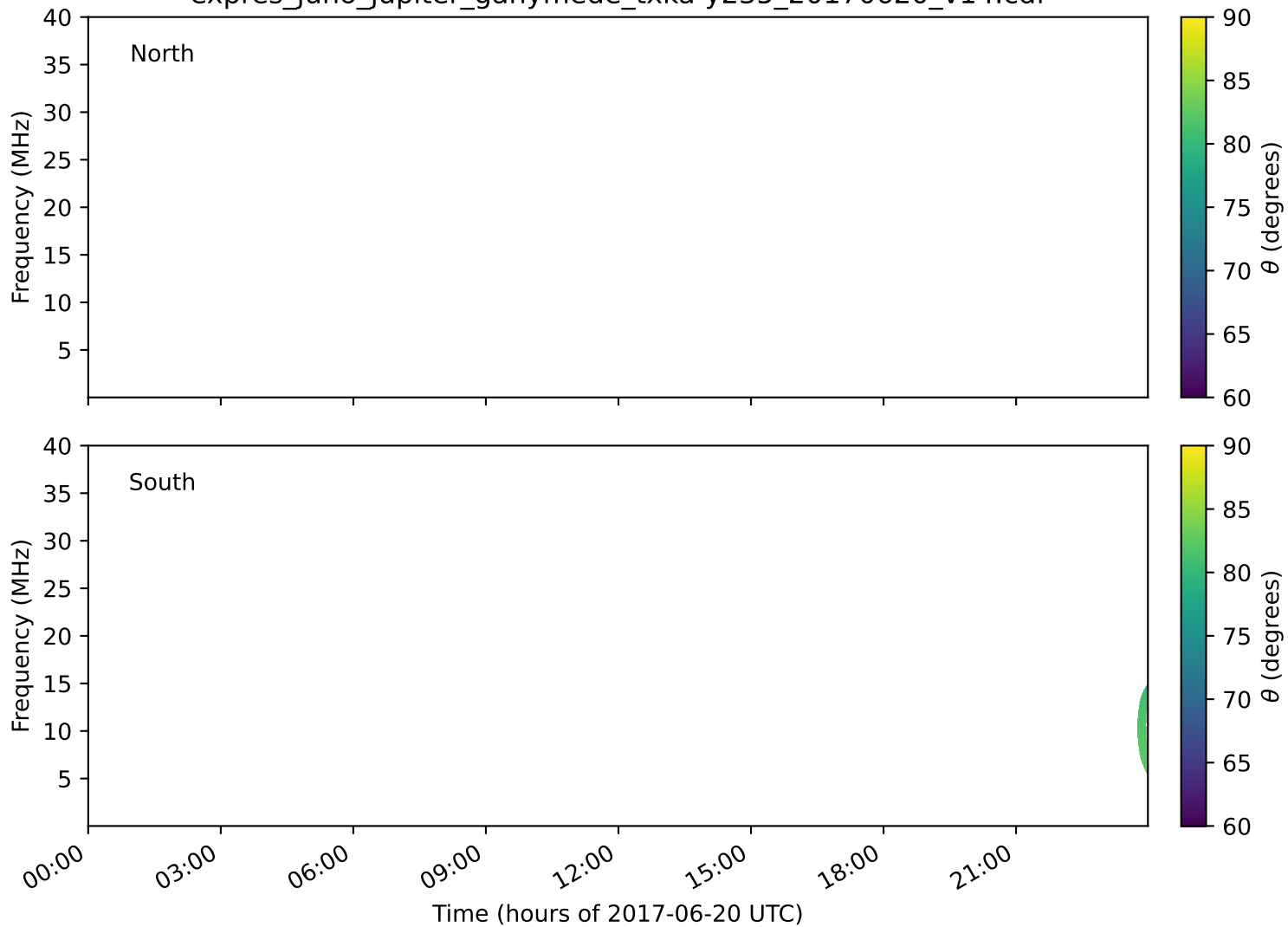
expres_juno_jupiter_ganymede_txka-y235_20170620_v14.cdf
