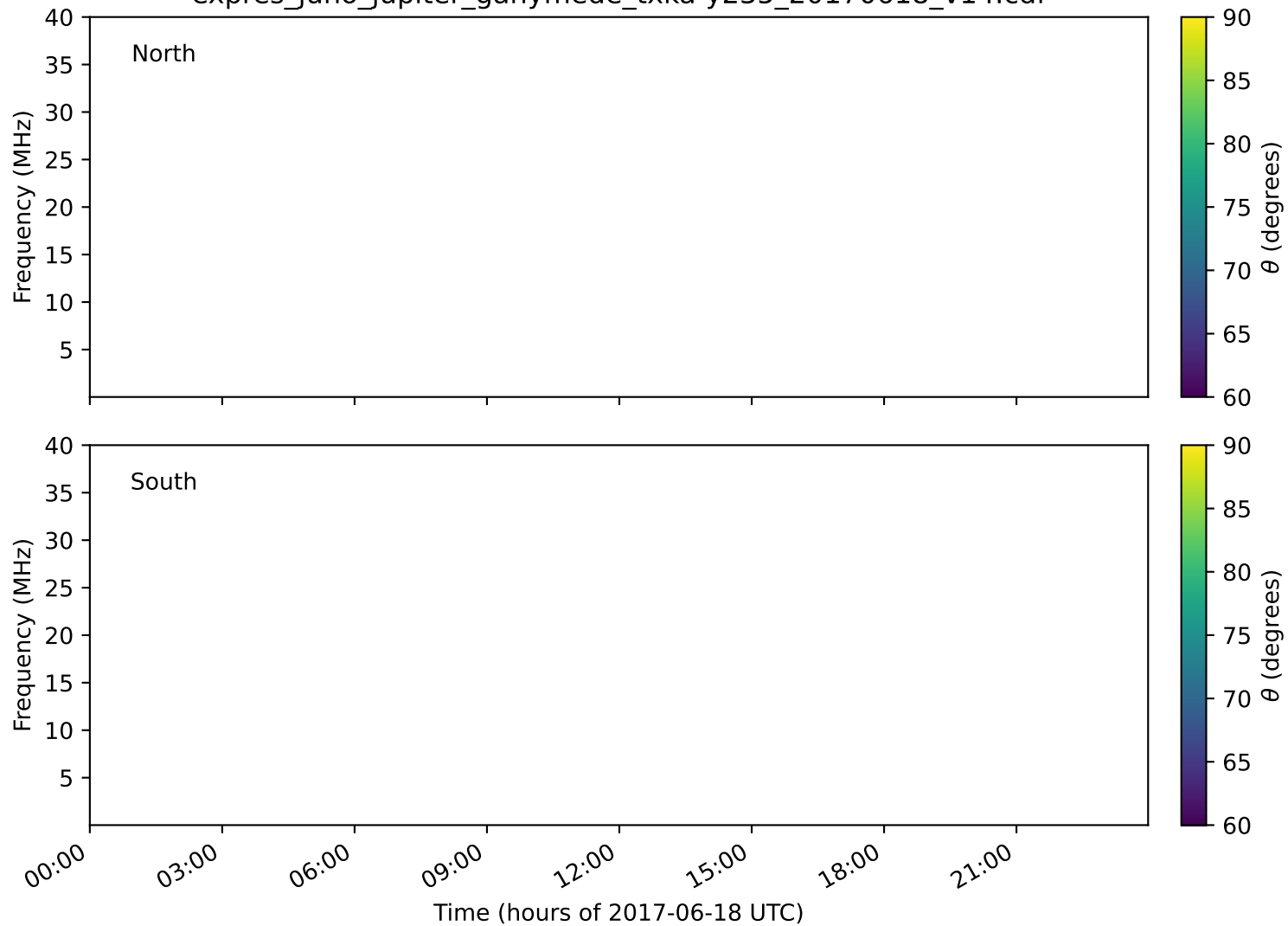
expres_juno_jupiter_ganymede_txka-y235_20170618_v14.cdf
