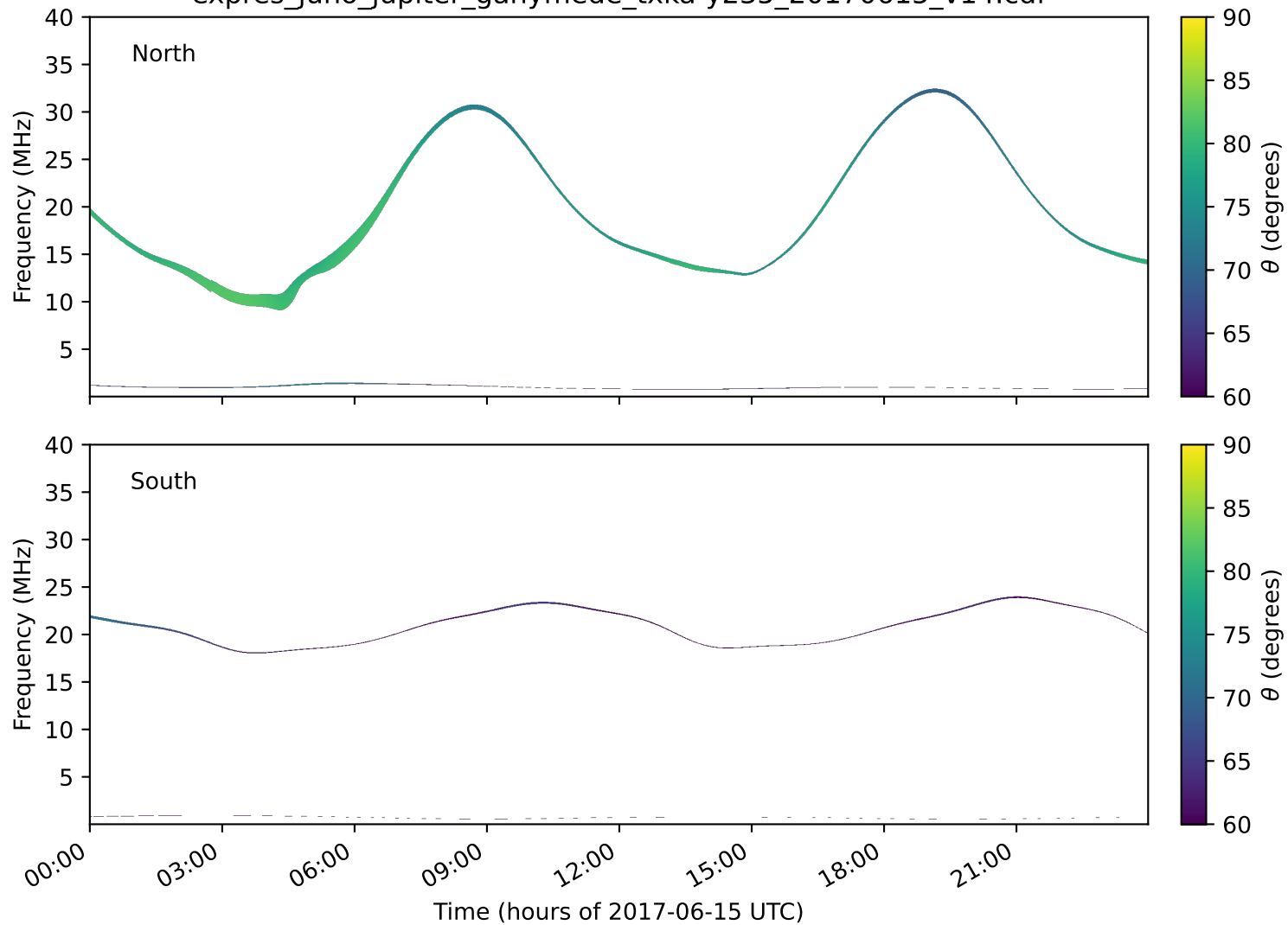
expres_juno_jupiter_ganymede_txka-y235_20170615_v14.cdf
