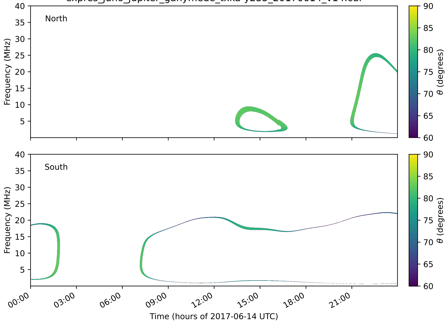
expres_juno_jupiter_ganymede_txka-y235_20170614_v14.cdf
