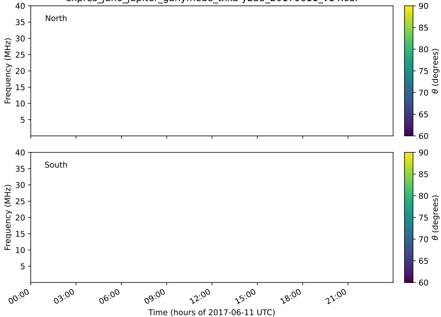
expres_juno_jupiter_ganymede_txka-y235_20170611_v14.cdf
