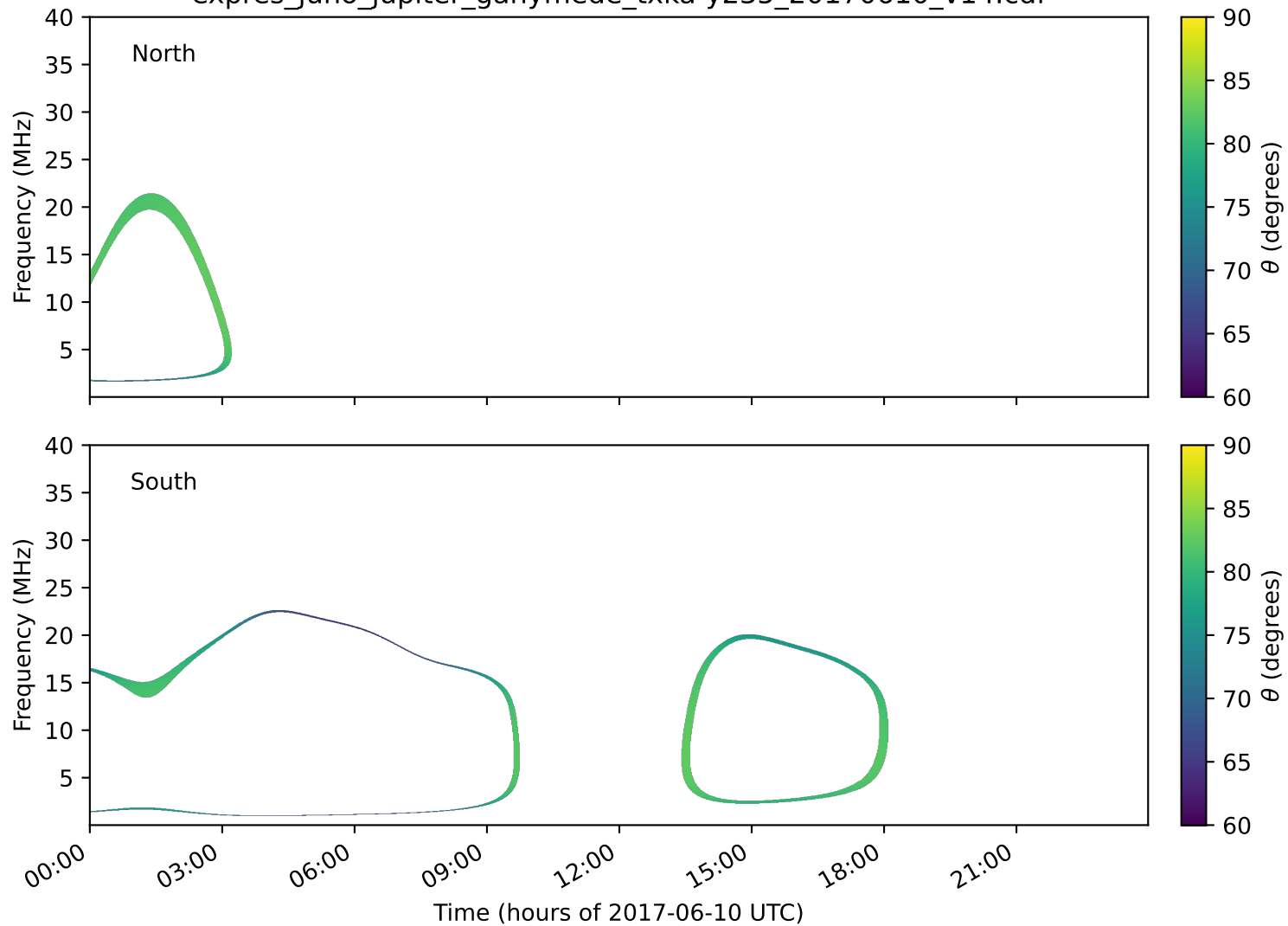
expres_juno_jupiter_ganymede_txka-y235_20170610_v14.cdf
