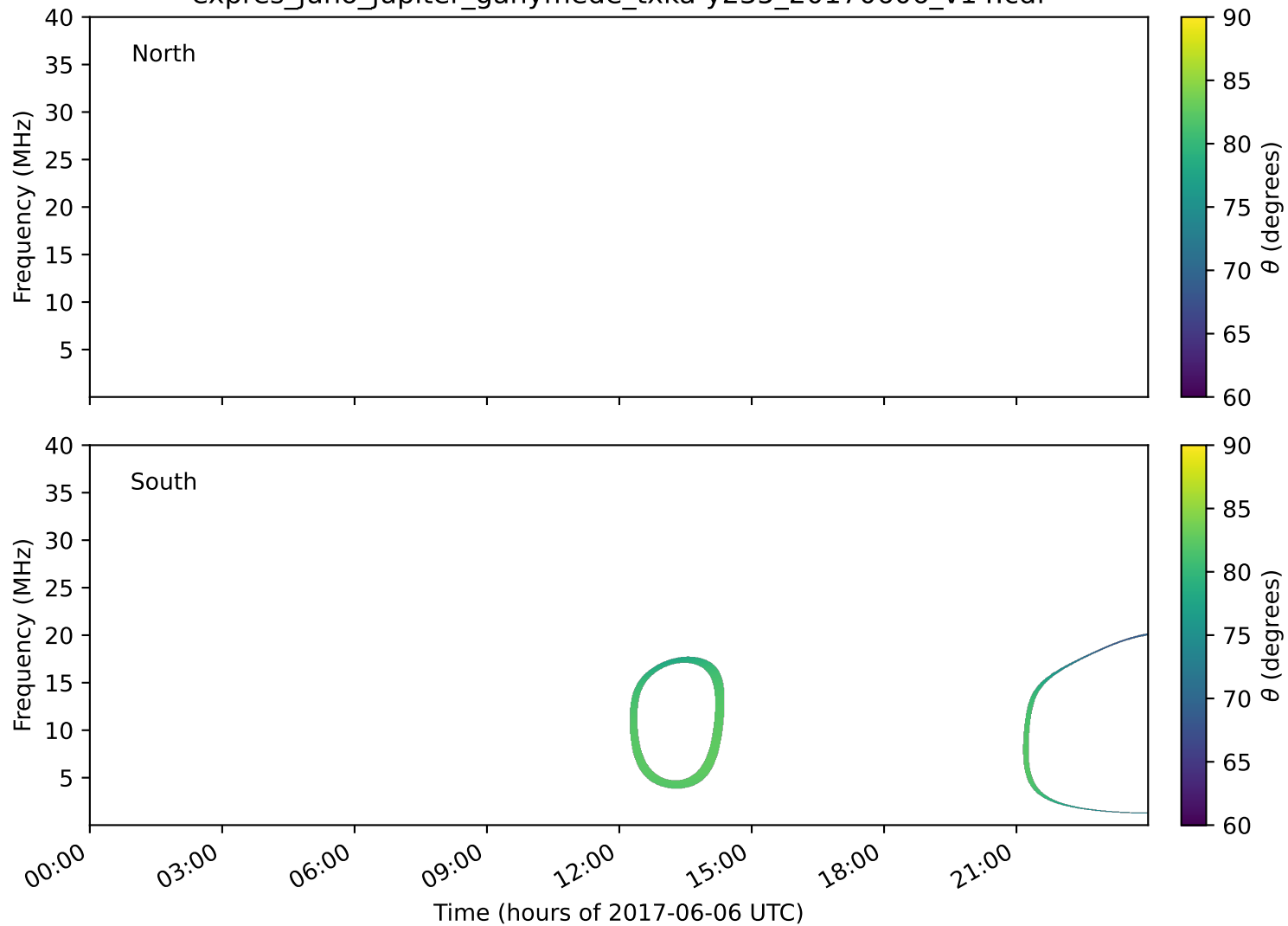
expres_juno_jupiter_ganymede_txka-y235_20170606_v14.cdf
