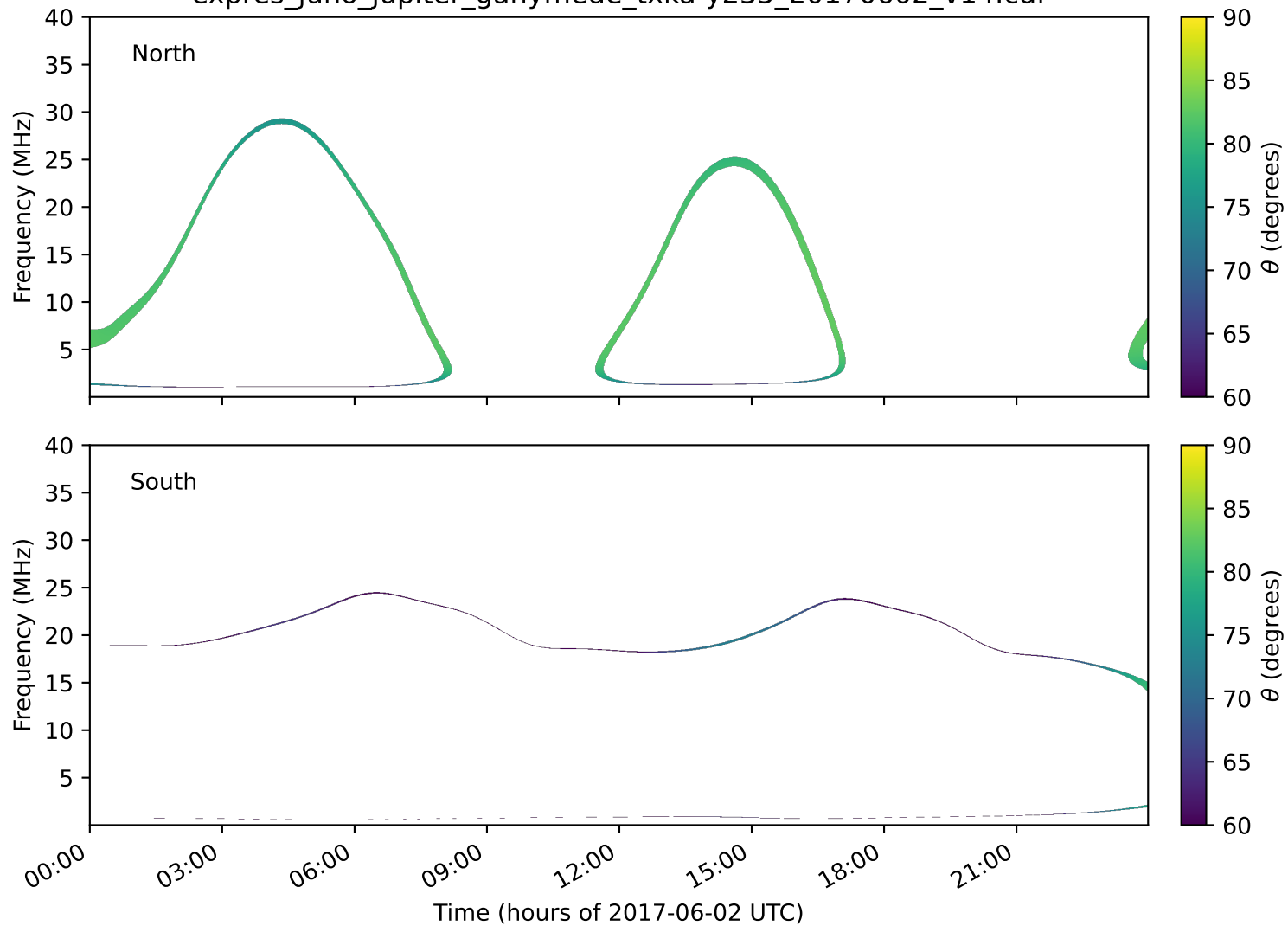
expres_juno_jupiter_ganymede_txka-y235_20170602_v14.cdf
