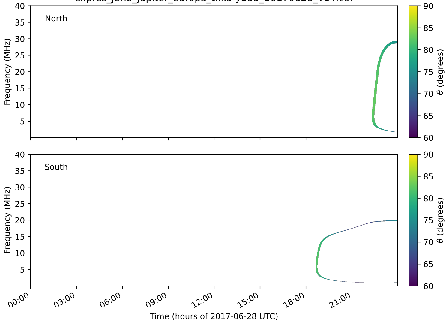
expres_juno_jupiter_europa_txka-y235_20170628_v14.cdf
