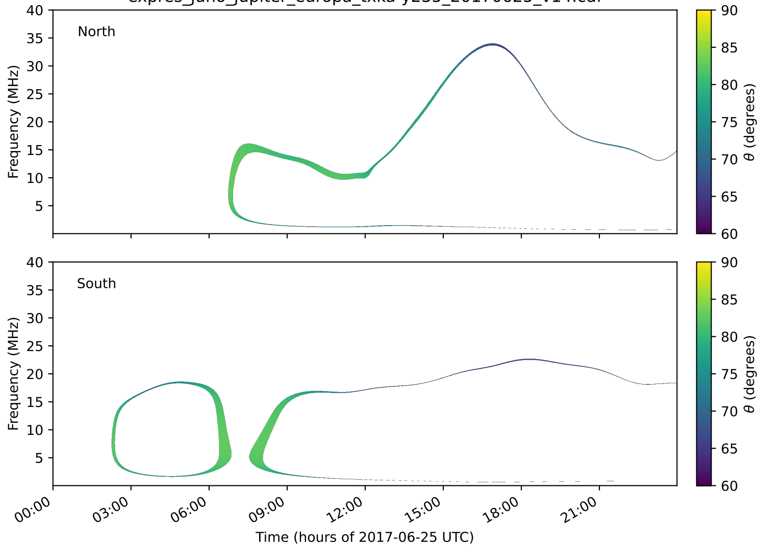
expres_juno_jupiter_europa_txka-y235_20170625_v14.cdf
