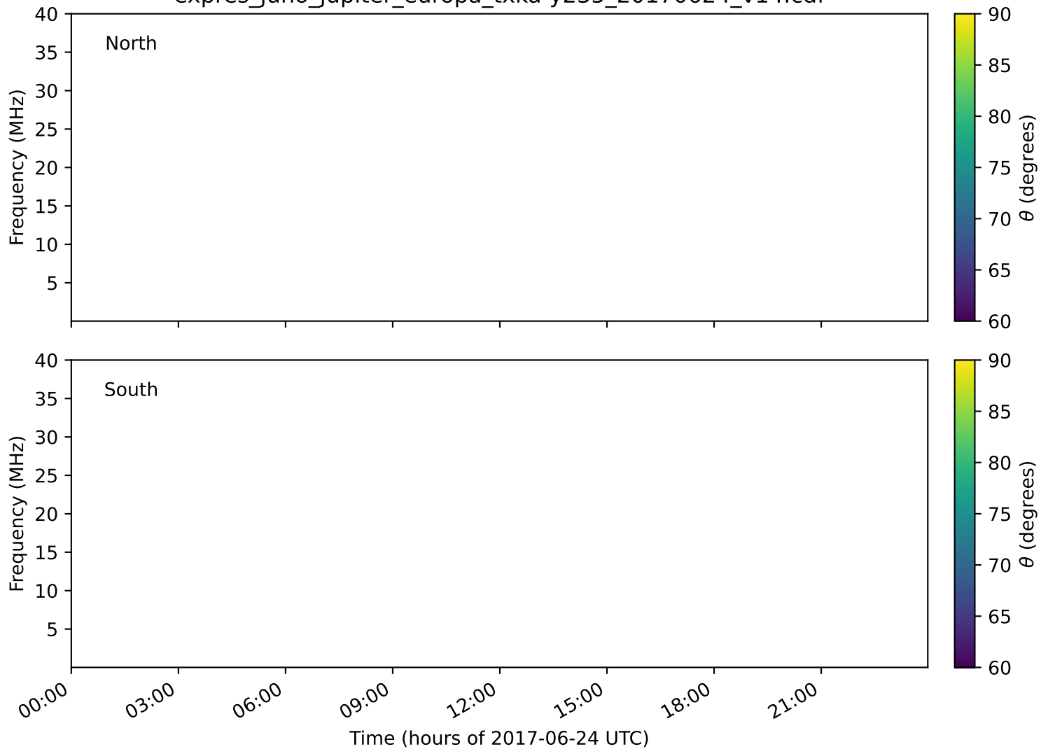
expres_juno_jupiter_europa_txka-y235_20170624_v14.cdf
