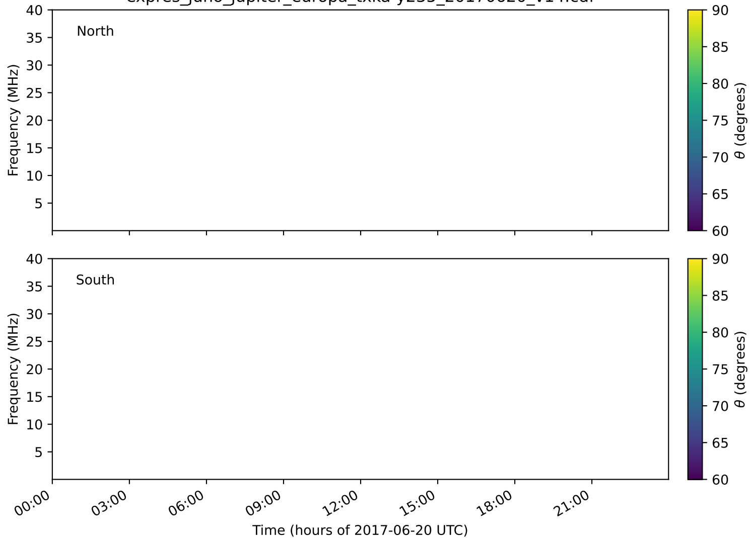
expres_juno_jupiter_europa_txka-y235_20170620_v14.cdf
