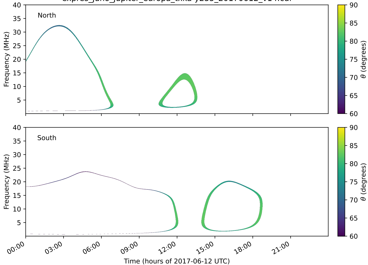
expres_juno_jupiter_europa_txka-y235_20170612_v14.cdf
