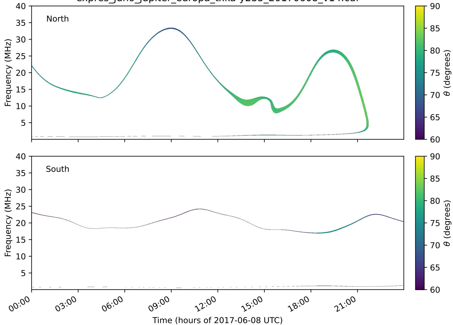
expres_juno_jupiter_europa_txka-y235_20170608_v14.cdf
