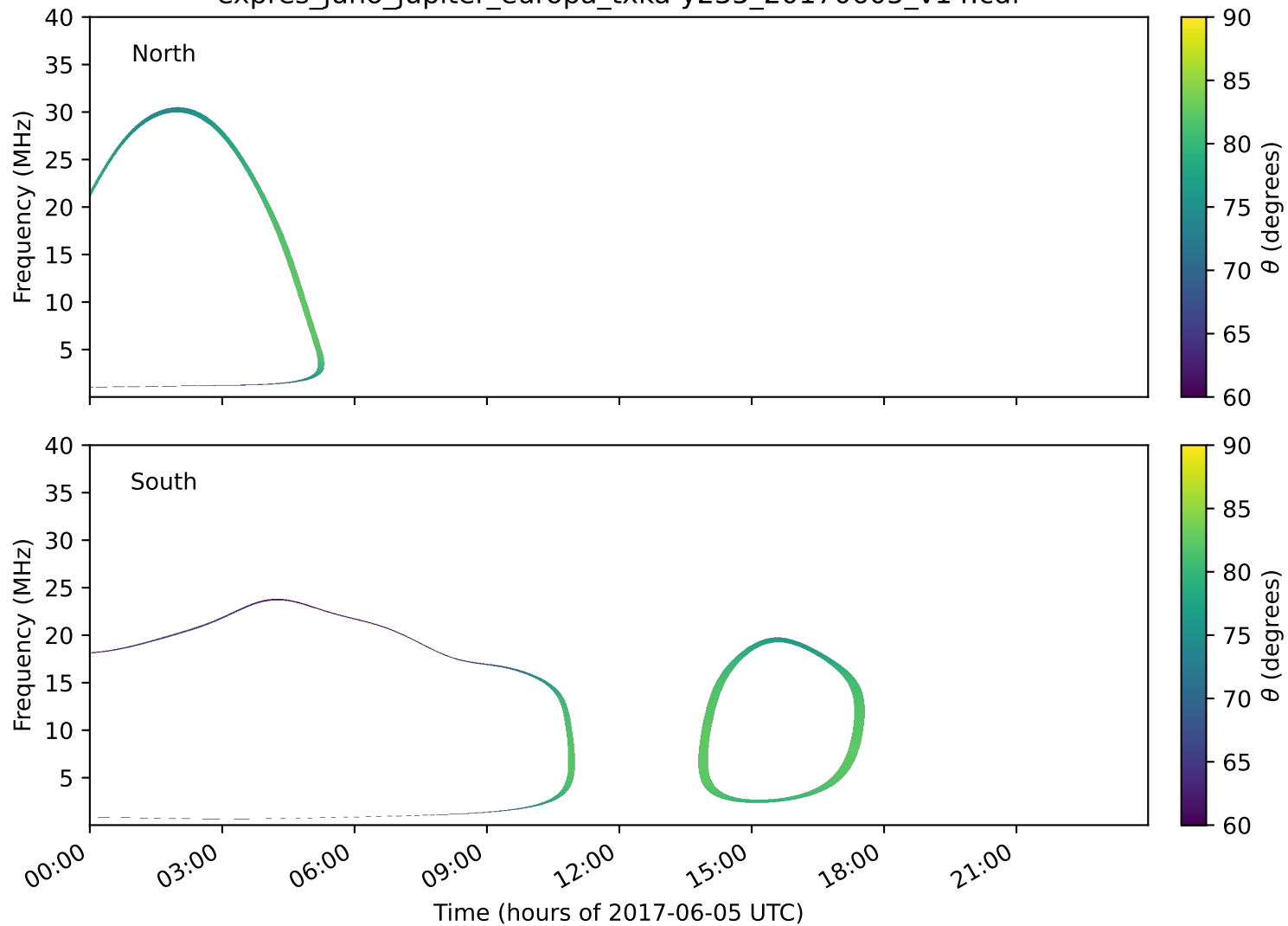
expres_juno_jupiter_europa_txka-y235_20170605_v14.cdf
