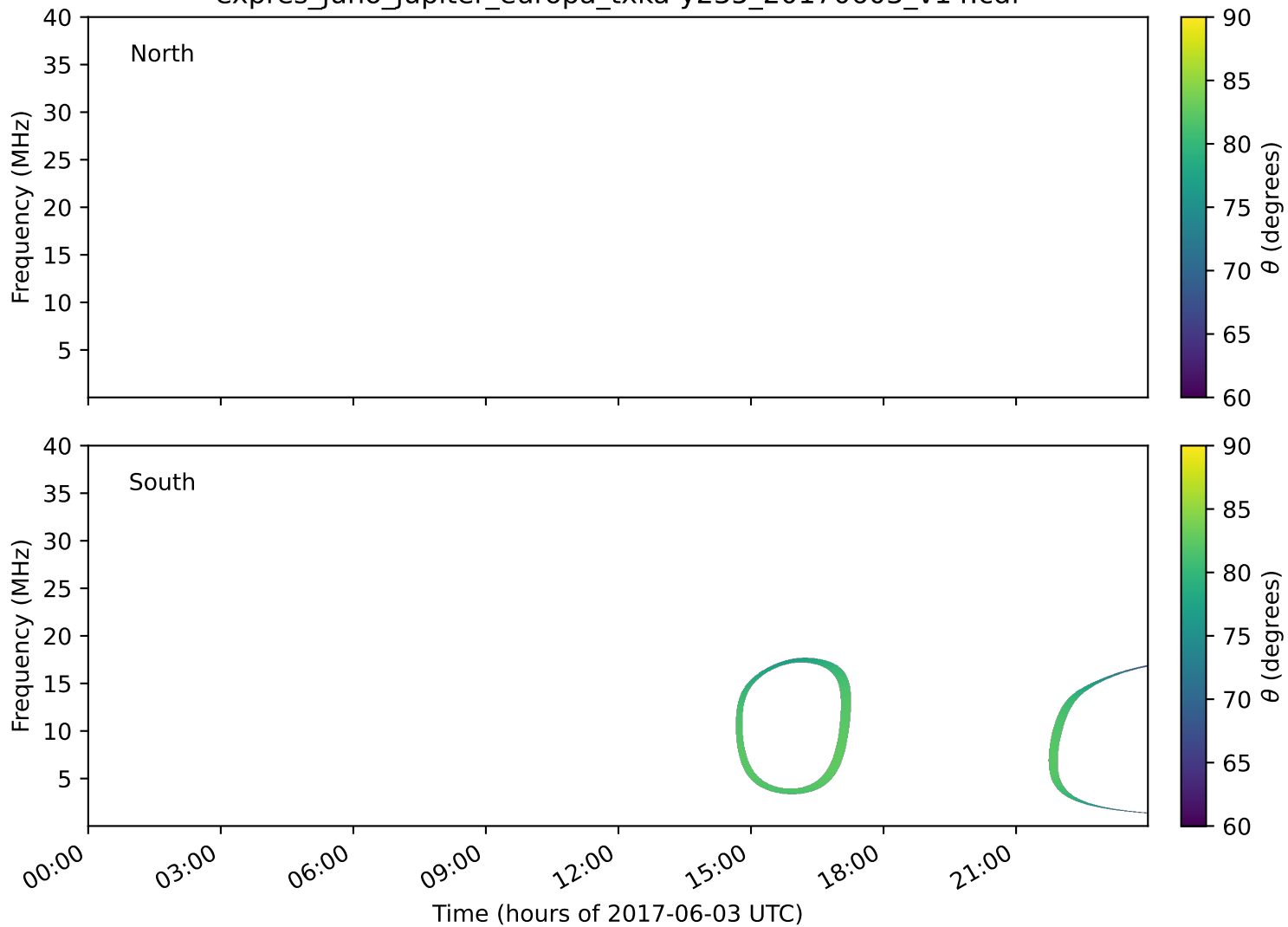
expres_juno_jupiter_europa_txka-y235_20170603_v14.cdf
