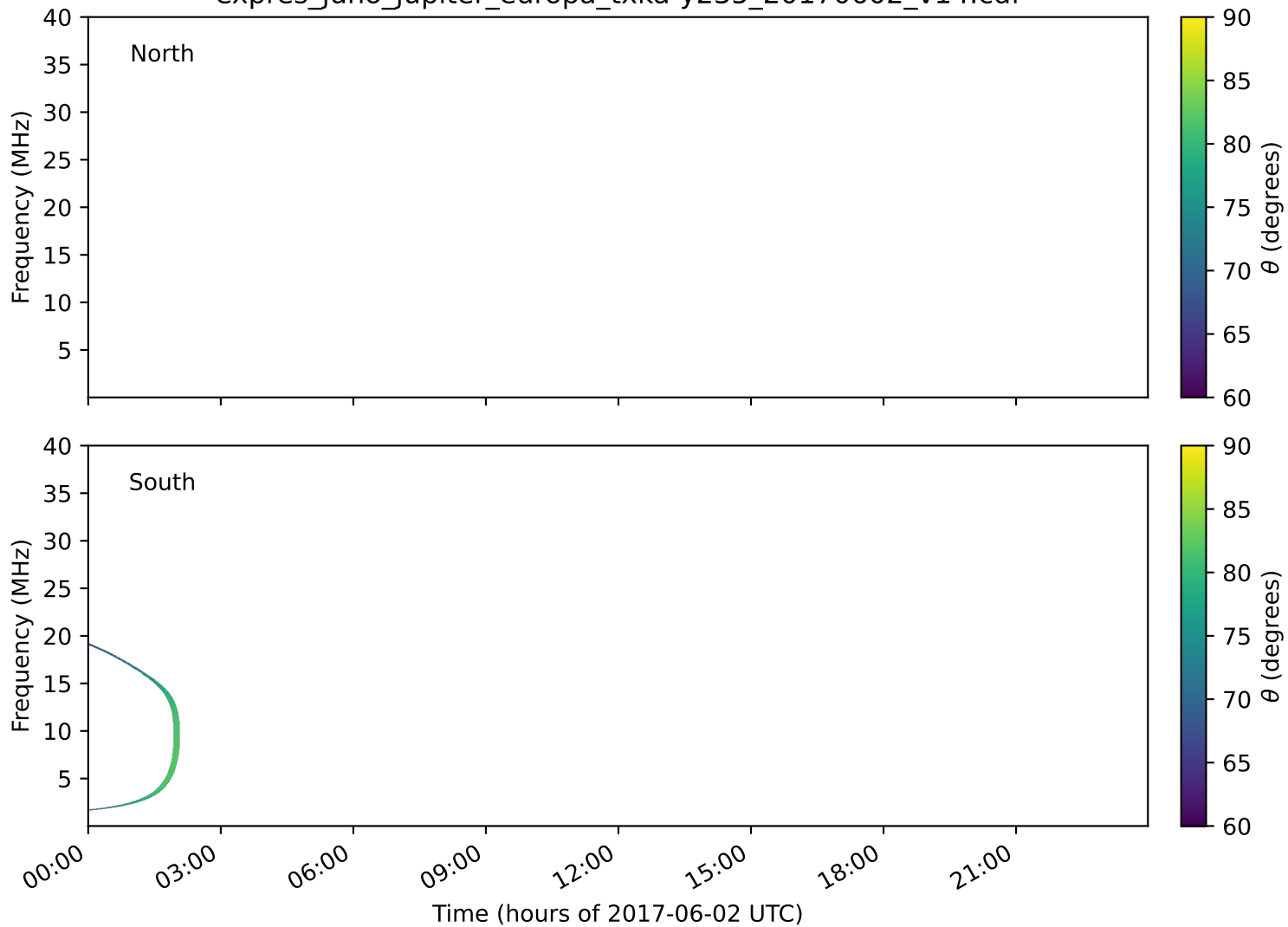
expres_juno_jupiter_europa_txka-y235_20170602_v14.cdf
