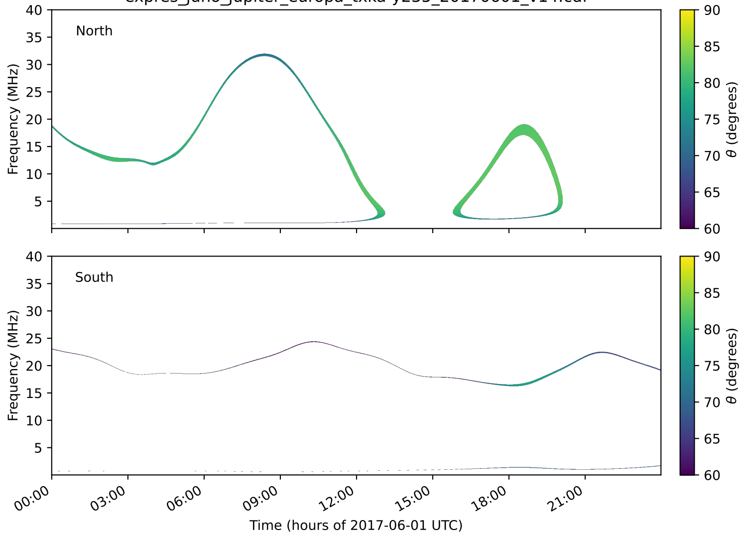
expres_juno_jupiter_europa_txka-y235_20170601_v14.cdf
