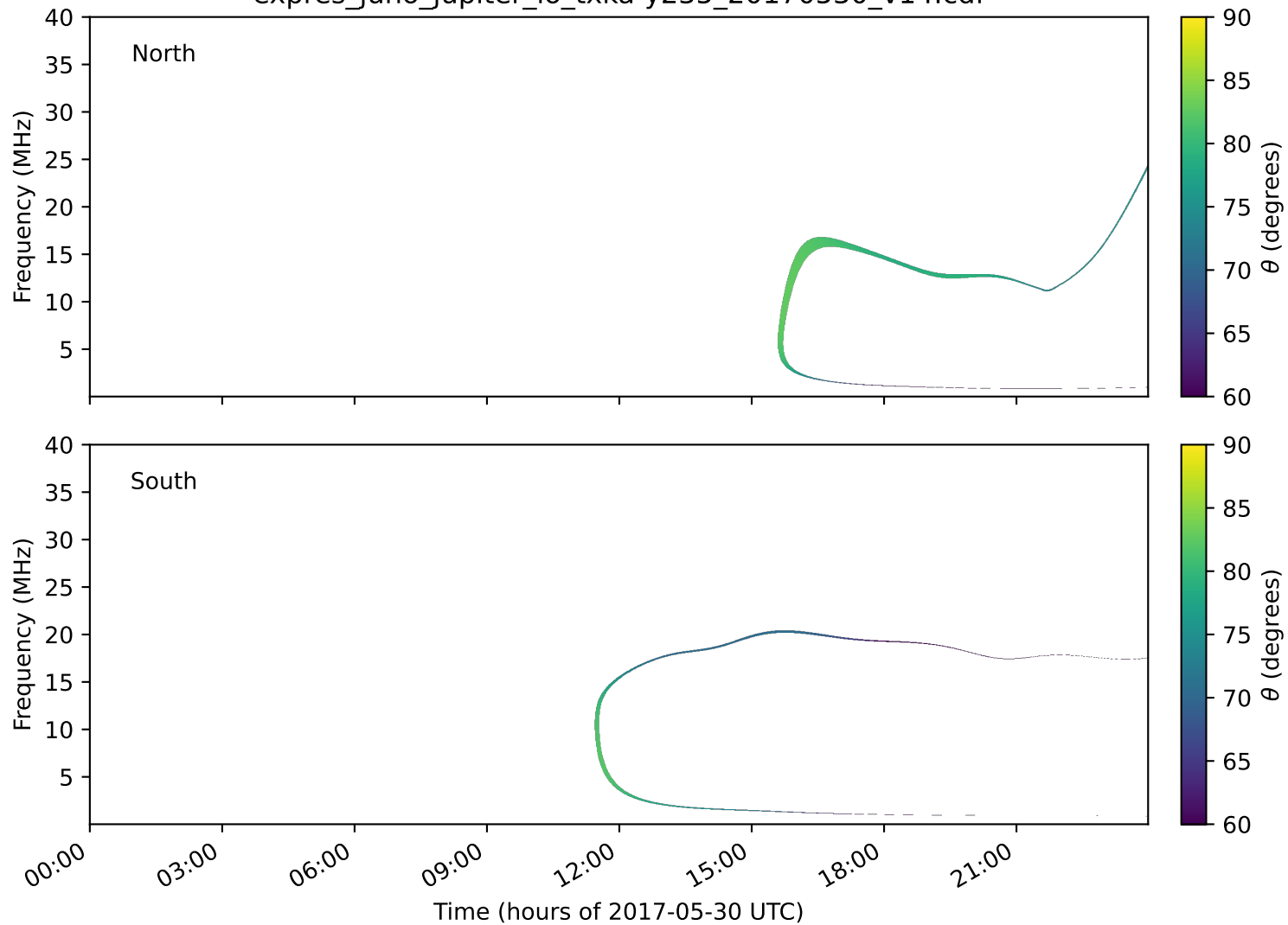
expres_juno_jupiter_io_txka-y235_20170530_v14.cdf
