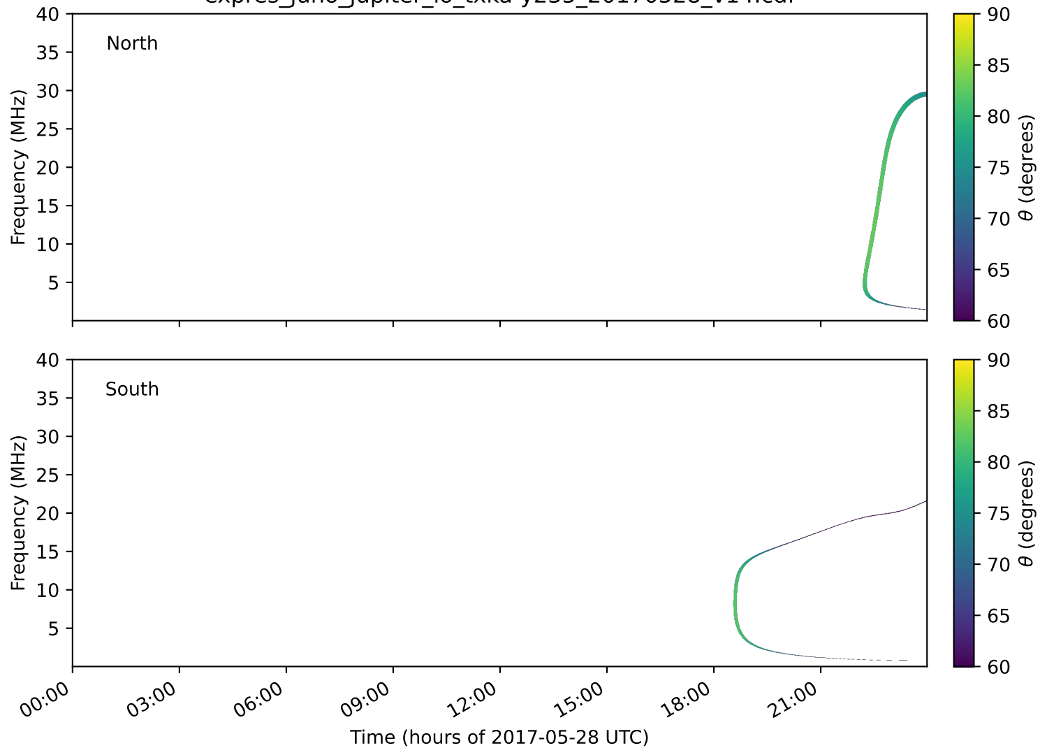
expres_juno_jupiter_io_txka-y235_20170528_v14.cdf
