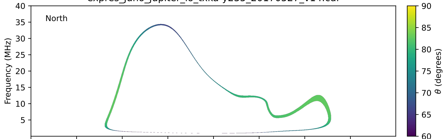
expres_juno_jupiter_io_txka-y235_20170527_v14.cdf
