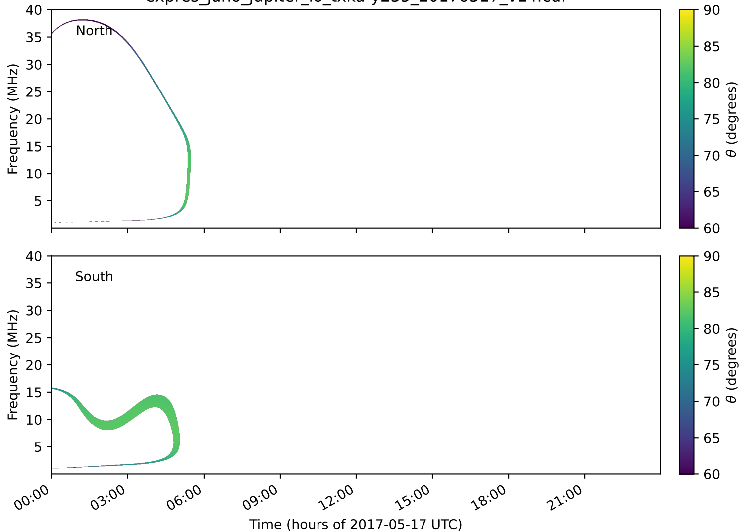
expres_juno_jupiter_io_txka-y235_20170517_v14.cdf
