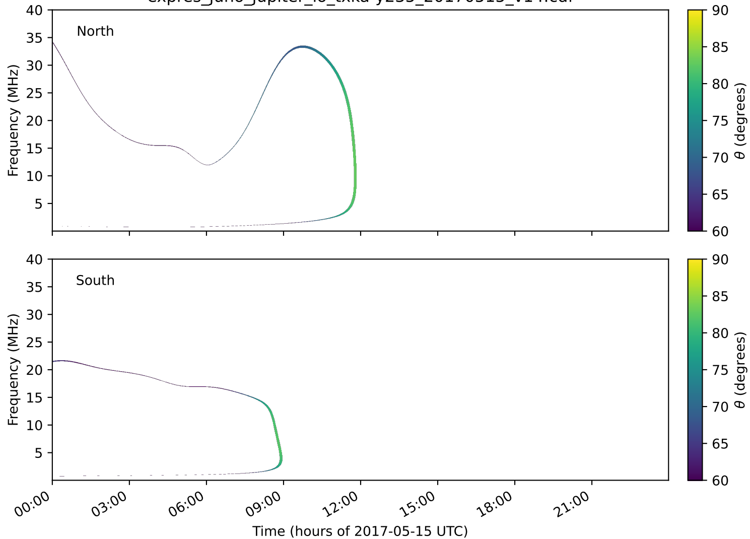
expres_juno_jupiter_io_txka-y235_20170515_v14.cdf
