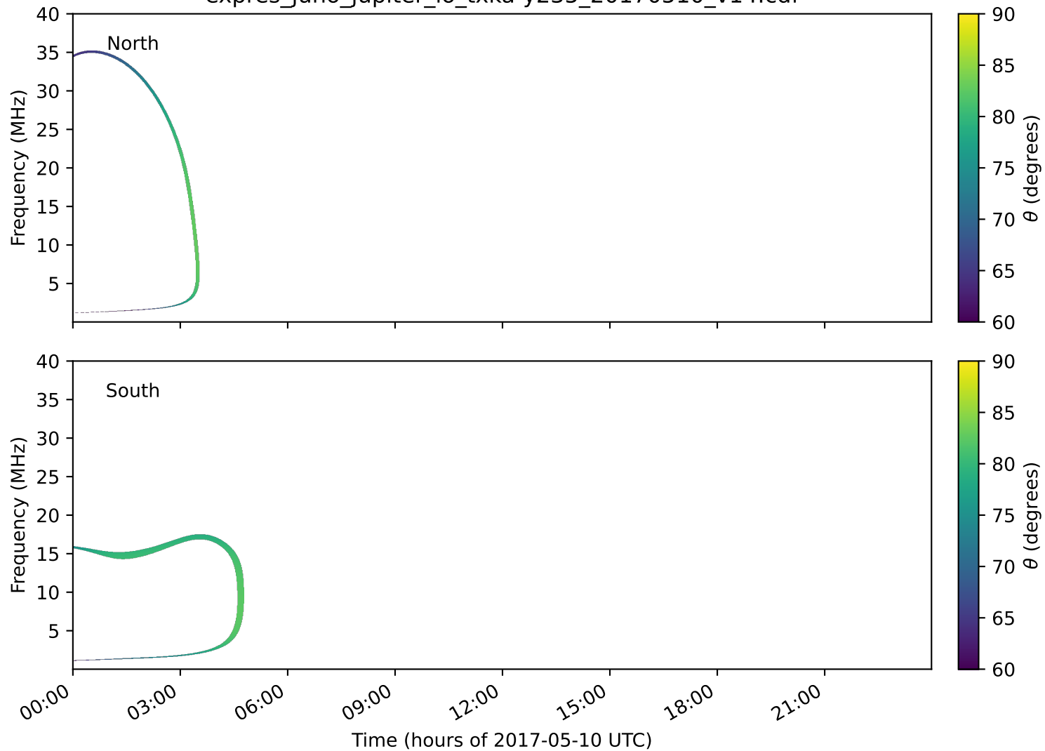
expres_juno_jupiter_io_txka-y235_20170510_v14.cdf
