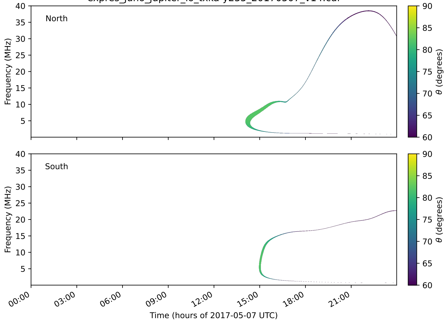
expres_juno_jupiter_io_txka-y235_20170507_v14.cdf
