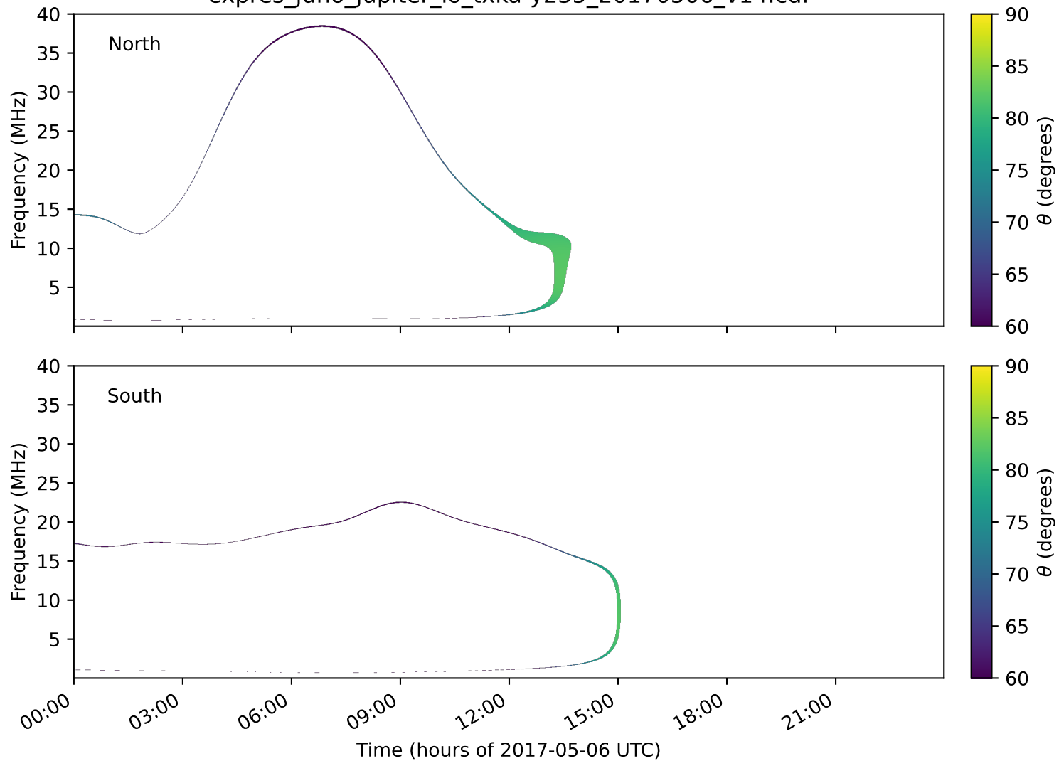
expres_juno_jupiter_io_txka-y235_20170506_v14.cdf
